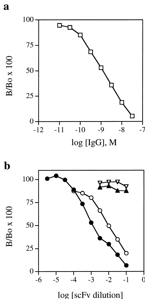
Fig. 4. AahII neutralizing capacities of IgG (a) and scFv-4C1 (b). Binding of [^{125}\text{I}]\text{AahII} ( 1 \times 10^{-10} M) to rat brain synaptosomes was inhibited by incubation with IgG (open square) or periplasmic (open circle) or culture supernatant (filled circle) scFv-4C1 preparations. Periplasmic (open triangle) and culture supernatant (filled triangle) scFv A58 preparations were used as a control. B and Bo are the binding measured with (B) or without (Bo) IgG or scFv.
